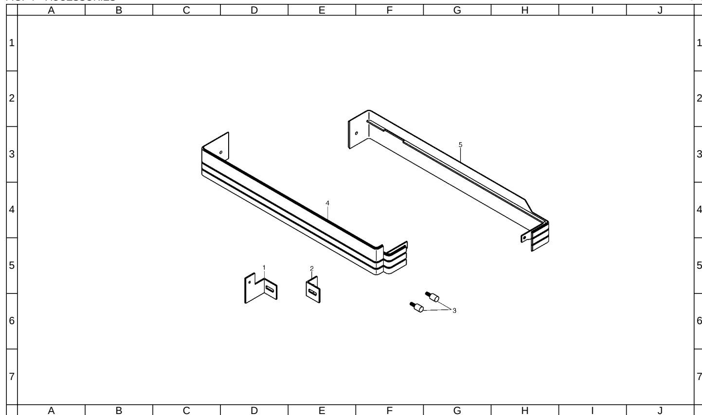
FIG. 4 ACCESSORIES
