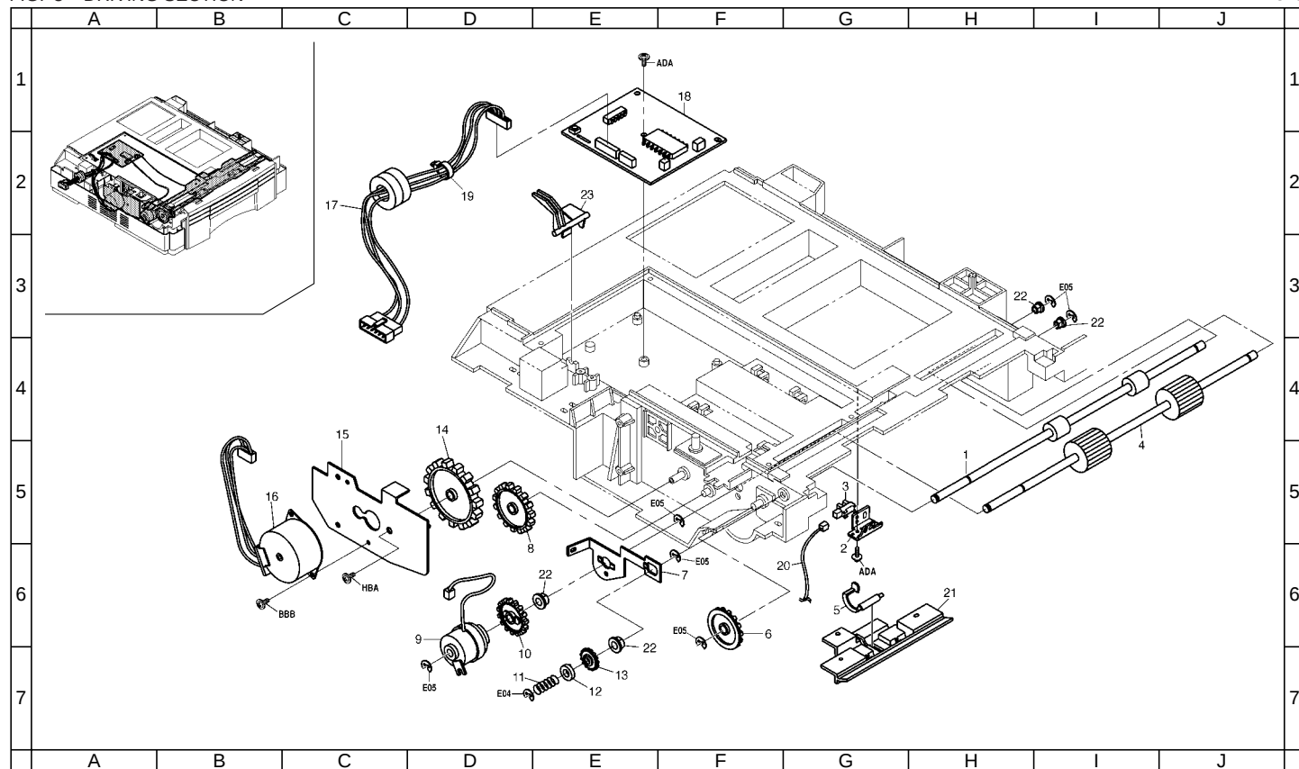
FIG. 3 DRIVING SECTION
